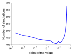
(d) Number of simulations for various \delta' , given an absolute error \epsilon = 0.1 , confidence parameter \delta = 0.05 and \gamma = 0.7 .
